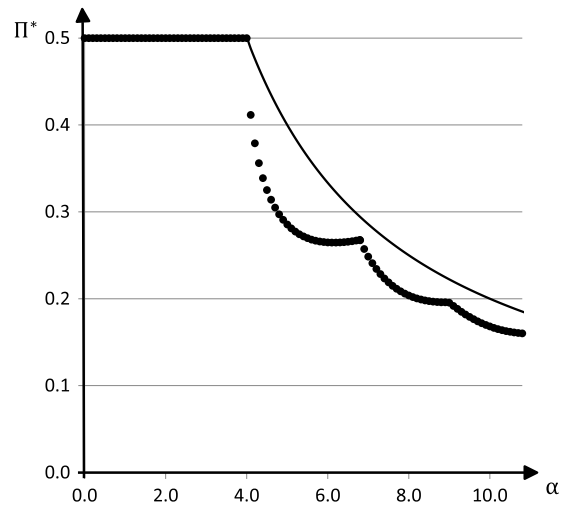
Fig. 1. Undissipated rent as a function of \alpha .
